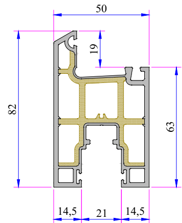
Sliding System Sash Profile
