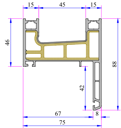
Penwood Frame Profile With Flat Sill
