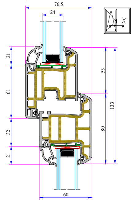
Mullion - Sash Installation
