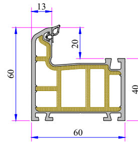
Frame Profile
