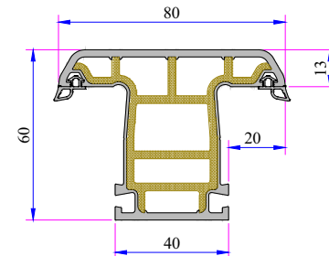
Mullion Profile
