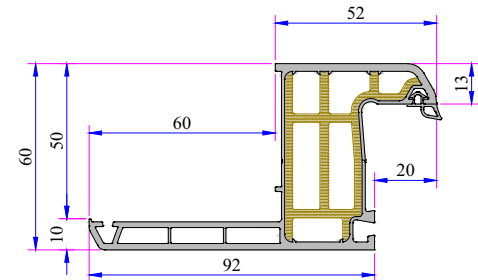
Frame With Sill Profile
