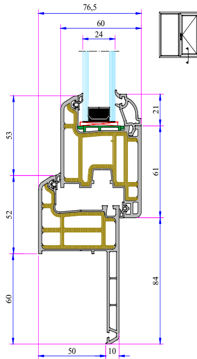
Frame With Sill - Sash Installation
