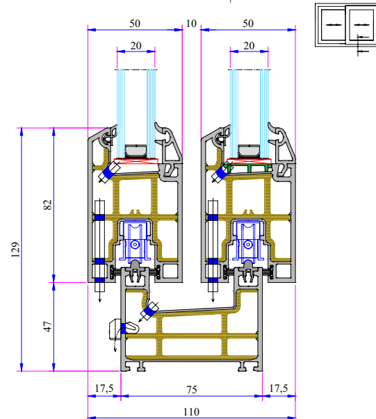
Sliding Frame Sash Double Rail Installation
