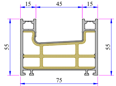
Penwood Frame Profile (Double Rail)
