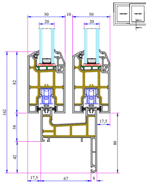
Double Sliding Frame with Sill - Sash Installation
