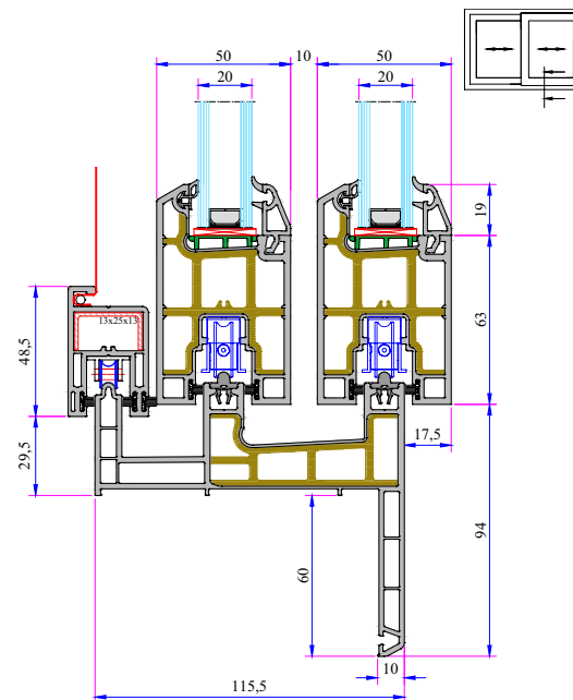
Double Sliding Frame with Sill (60mm) - Sash Installation
