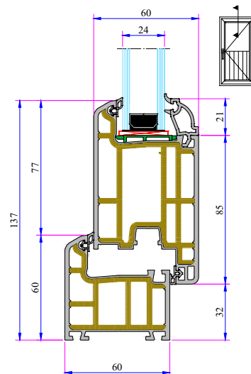
Frame - Door Sash Installation
