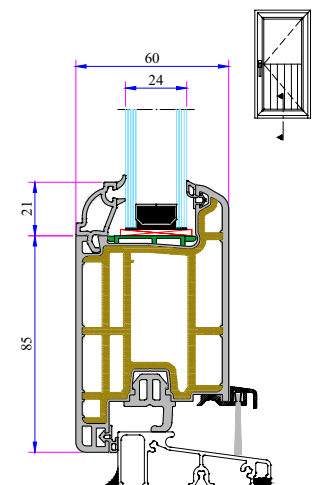
With Aluminium Threshold Frame Door Sash Installation
