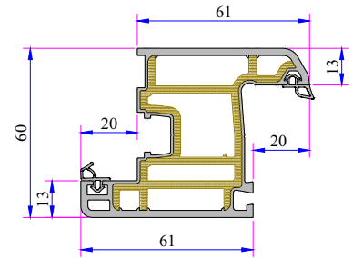
Sash Profile
